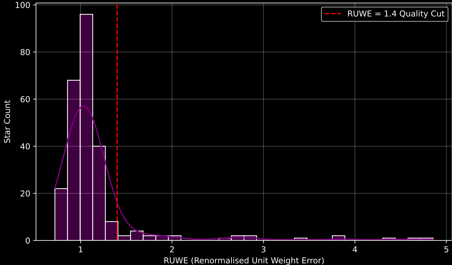
GALAH DR4 Field [7171] RUWE Distribution (n= 257)
