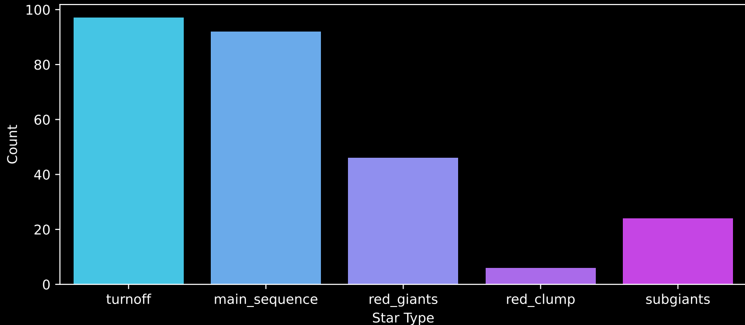
GALAH DR4 Field: [7171] Count plot of Star Type
