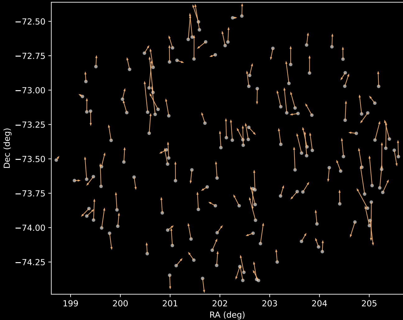
GALAH DR4 Cluster 3 Proper Motion Vectors (n=145)
